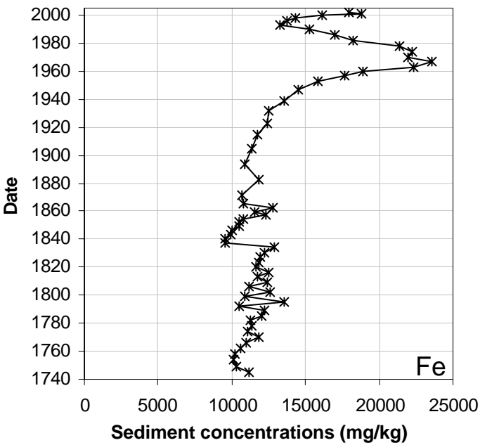
Fig. 13. Sediment concentration (mg/kg) profiles of cadmium (Cd), copper (Cu), lead (Pb) zinc (Zn) and iron (Fe) in Imp Lake.
