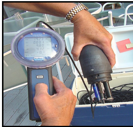
Hydrolab with receiving apparatus
